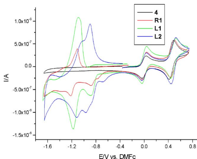
Fig. 4 CVs of compound 4 , R1 , L1 and L2 recorded in 0.10 \text{ M } n\text{Bu}_4\text{NPF}_6 in acetonitrile at a scan rate of 100 \text{ mV s}^{-1} .
