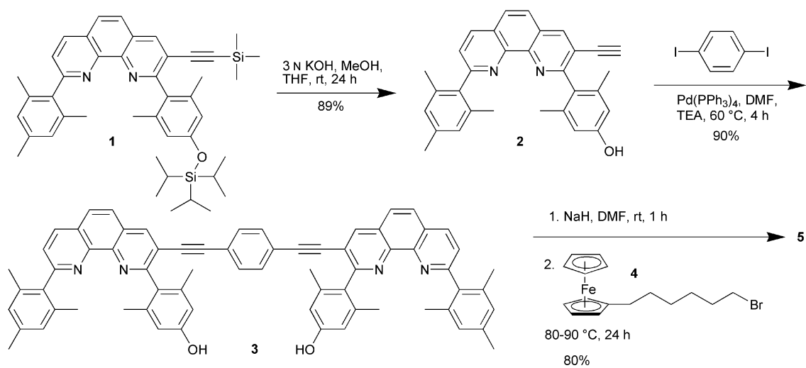
Scheme 2 Preparation of 5.
