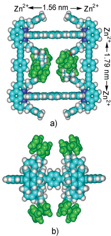
Fig. 1 Side (a) and top (b) views of space-filling presentations of nanoladder L2 [Zn_4(5)_2(7)_2]^{8+} as generated from force field modelling (HyperChem ® ). The atoms/groups are colour coded for clarity: carbon: cyan; nitrogen: blue; oxygen: red; zinc: (hidden); ferrocene group: green.
